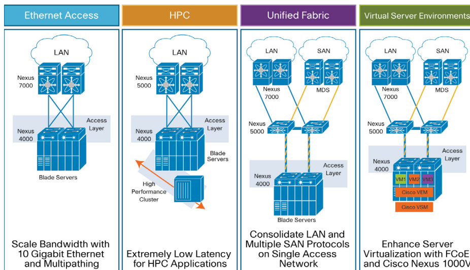
Figure 2. Four Data Center Solutions in One Switch - Deployment Scenarios for the Cisco Nexus 4001I
